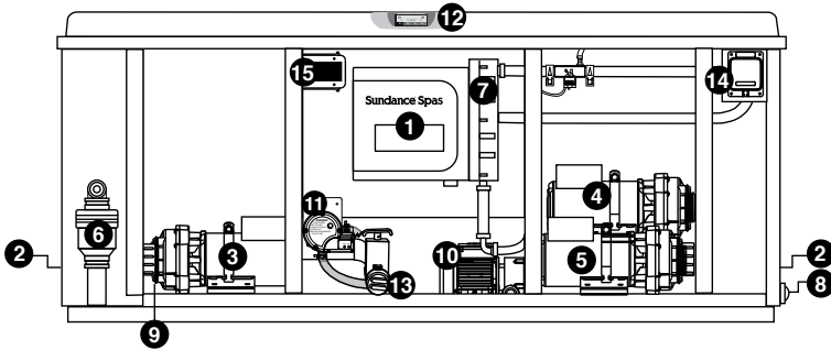
Figure A (Equipment Area for Maxxus/Aspen Models)
